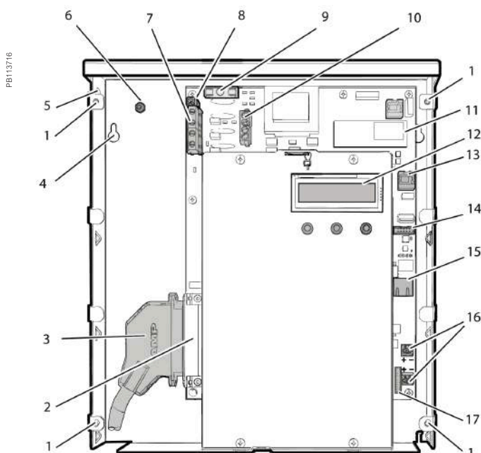
PowerLogic™ EM4033 and PowerLogic™ EM4080 internal view.
