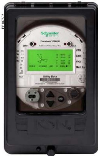
PowerLogic™ ION8650 meter with switchboard case
