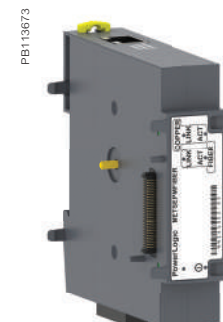
Fiber-Ethernet Option Module
