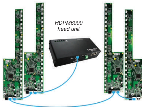
Metering Architecture
